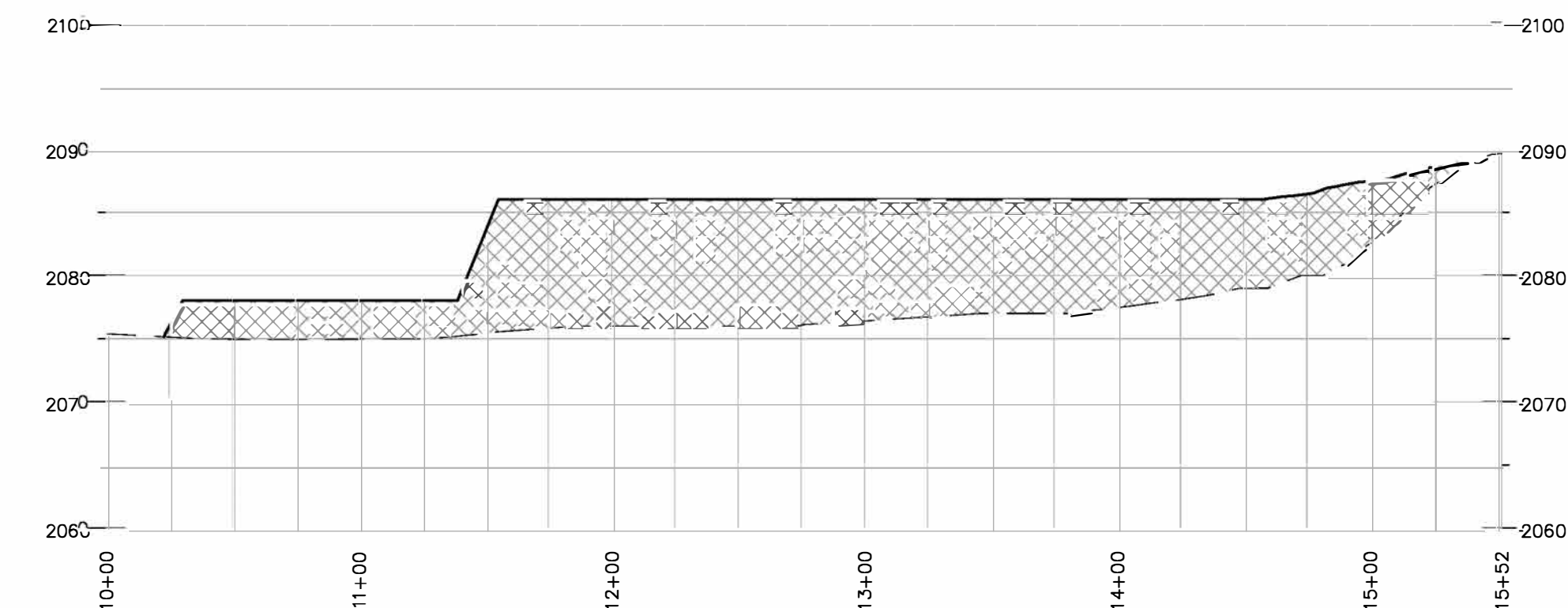
SECTION A
