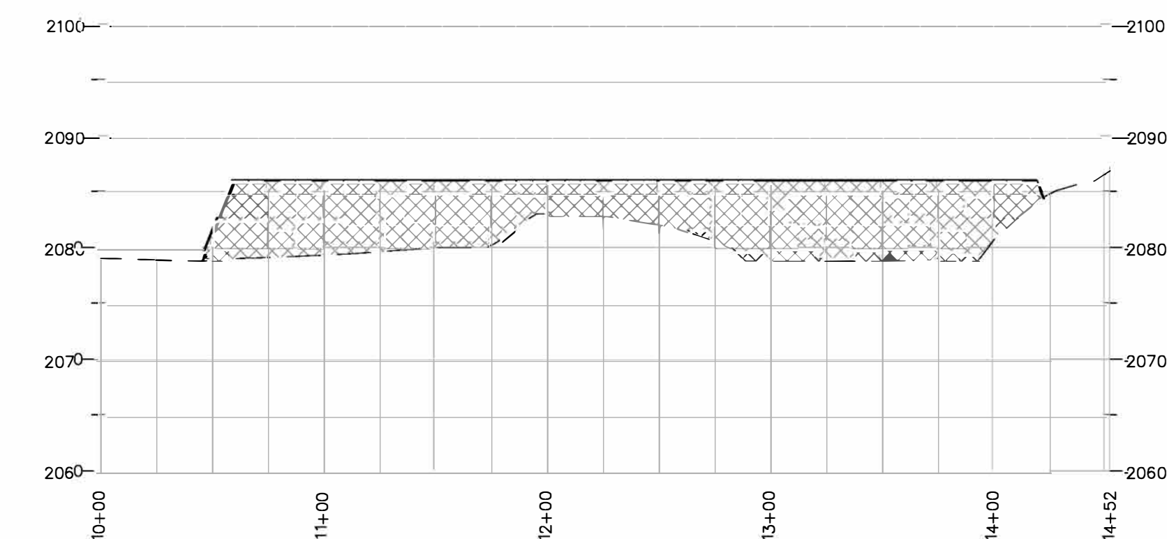
SECTION B
