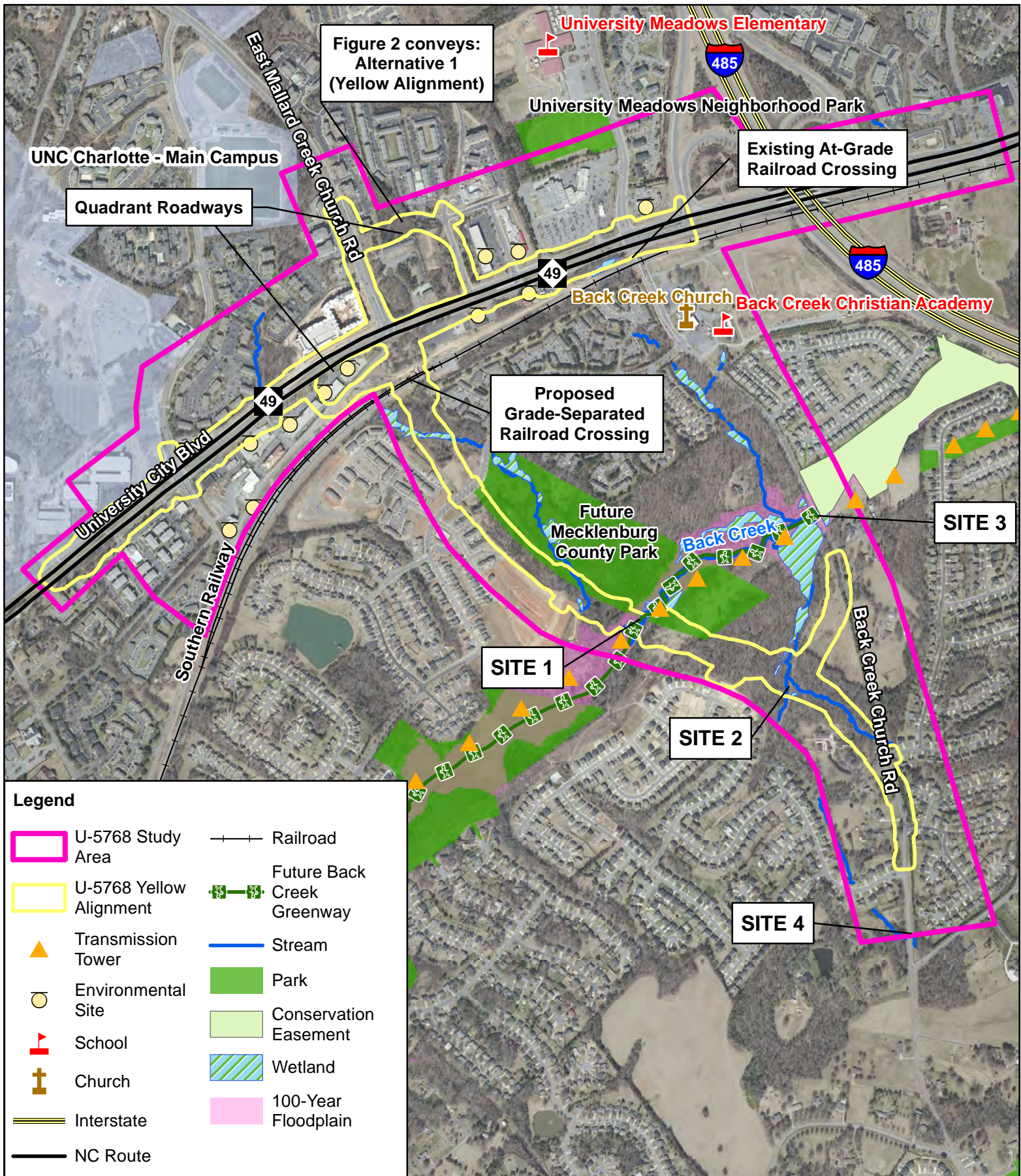
FIGURE 2 (Alternative 1) STIP U-5768 NC 49 Widening and Back Creek Church Road Realignment Charlotte, Mecklenburg County June 2019
