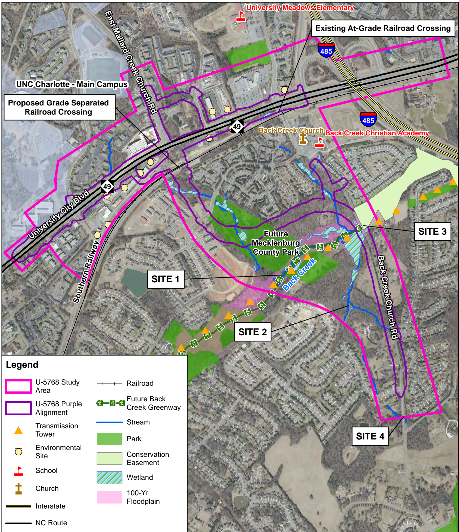
FIGURE 3 (Alternative 2) STIP U-5768 NC 49 Widening and Back Creek Church Road Realignment Charlotte, Mecklenburg County June, 2019
