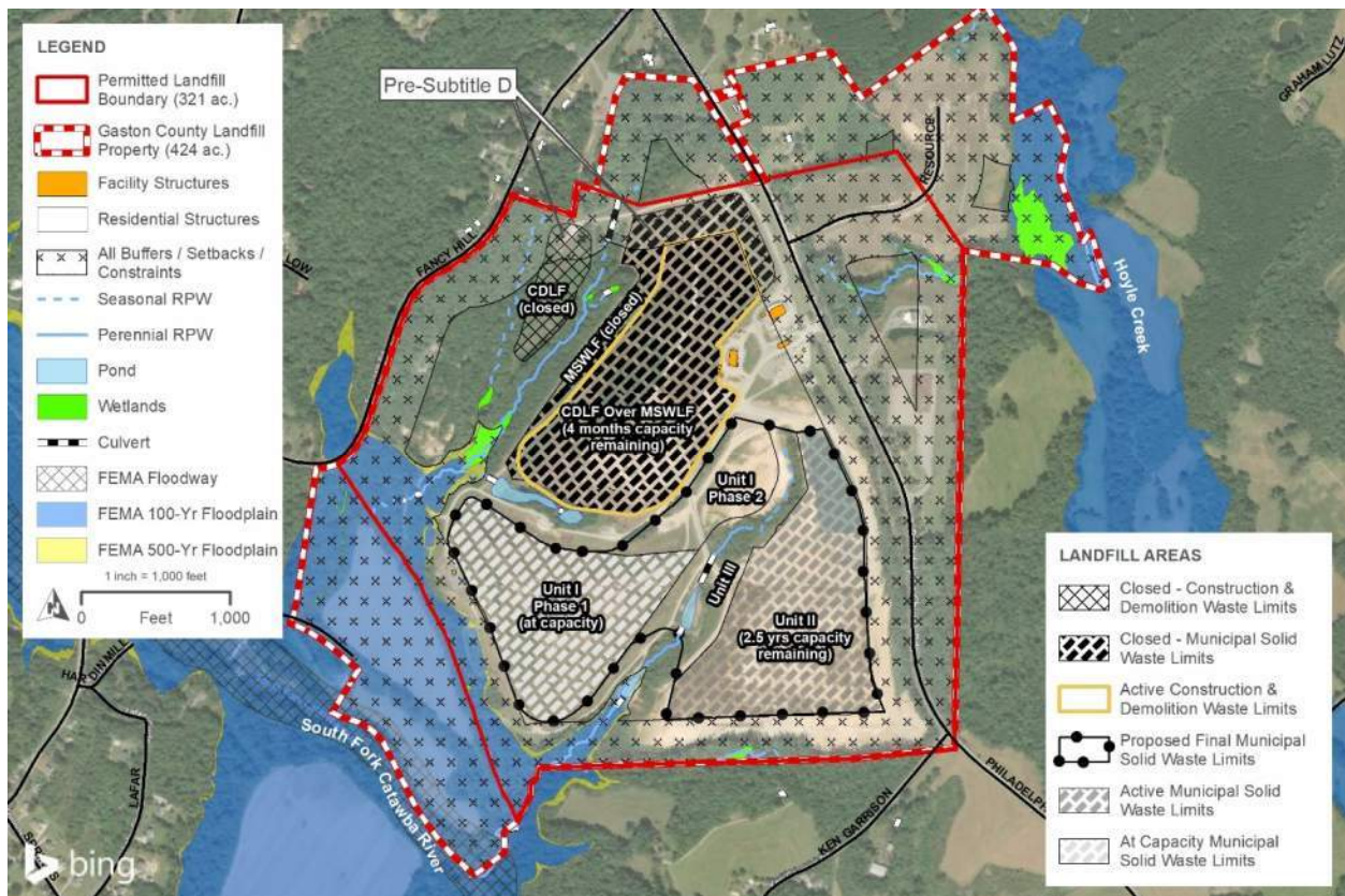
Figure 4. Gaston County Landfill Site Layout
