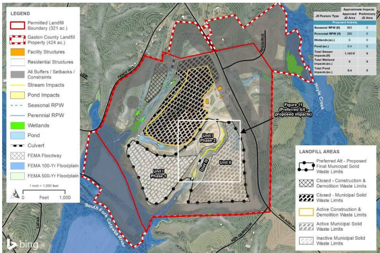
Figure 5. Preferred Alternative Site Layout – Impacts Overview
