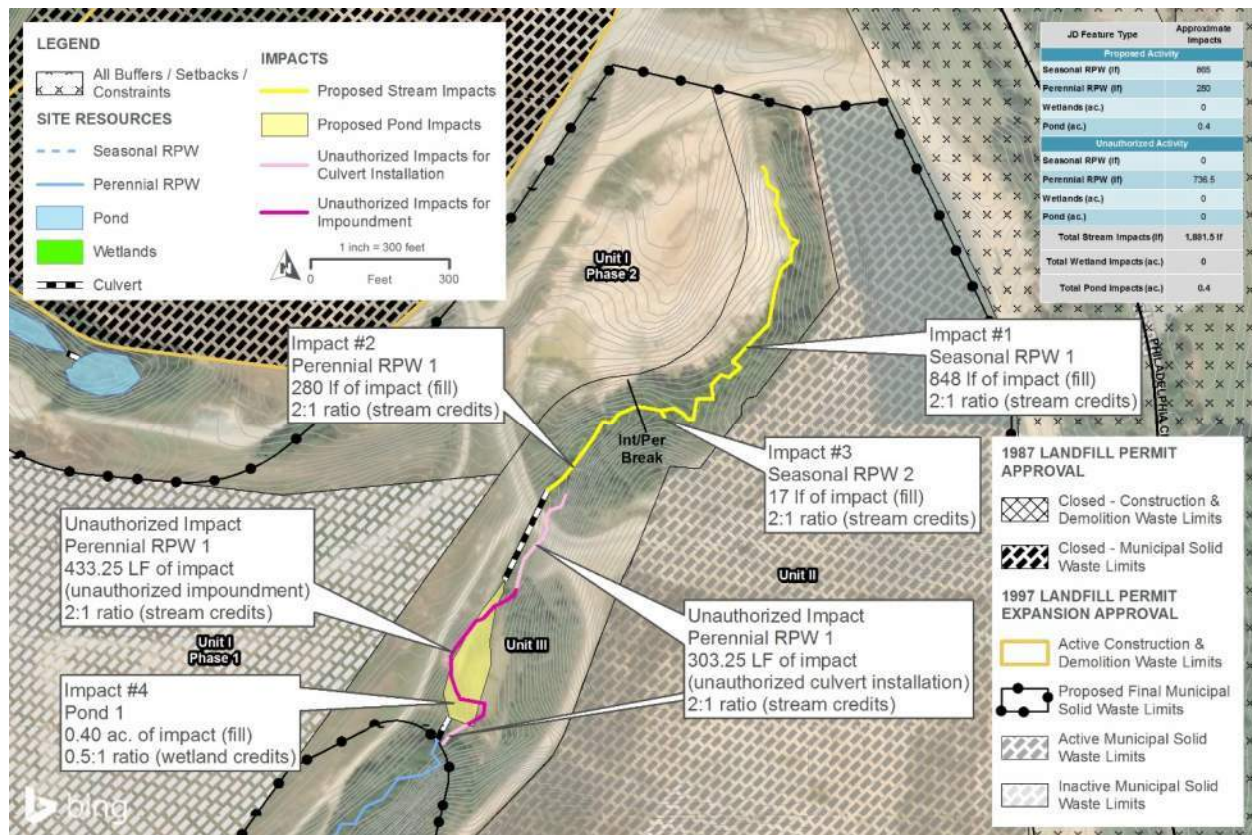
Figure 7. Proposed Impacts and Unauthorized Impacts that Previously Occurred
