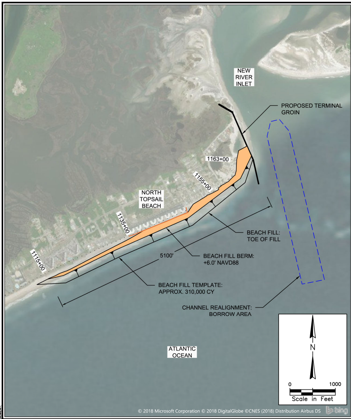
FIGURE 2: BEACH FILL TEMPLATE & TERMINAL GROIN North Topsail Beach Onslow County, NC April 11, 2018
