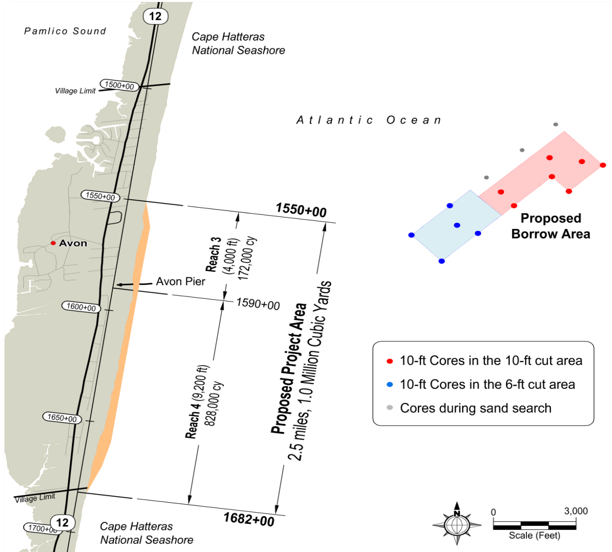
Figure 2. Plan view for the proposed project within the Village of Avon including the including the project limits, main placement area and borrow areas.
