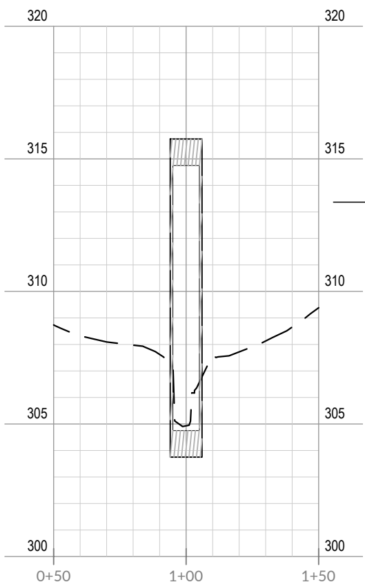
CULVERT DOWNSTREAM INVERT
