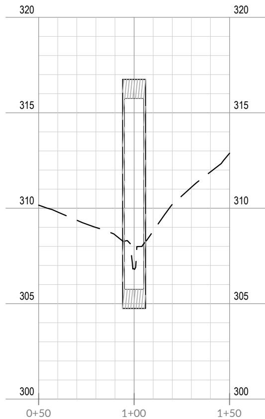
CULVERT UPSTREAM INVERT
