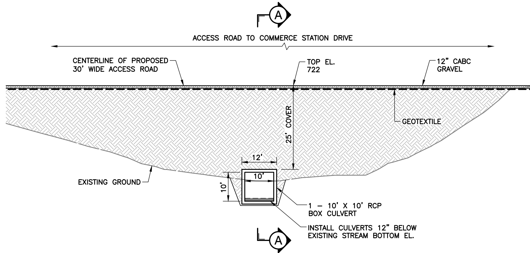
CULVERT CROSSING SECTION
