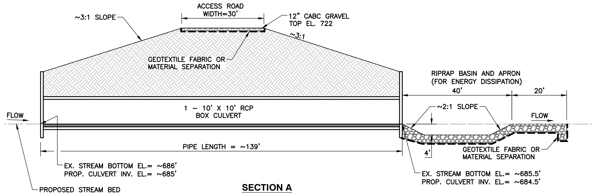
CULVERT CROSSING SECTION
