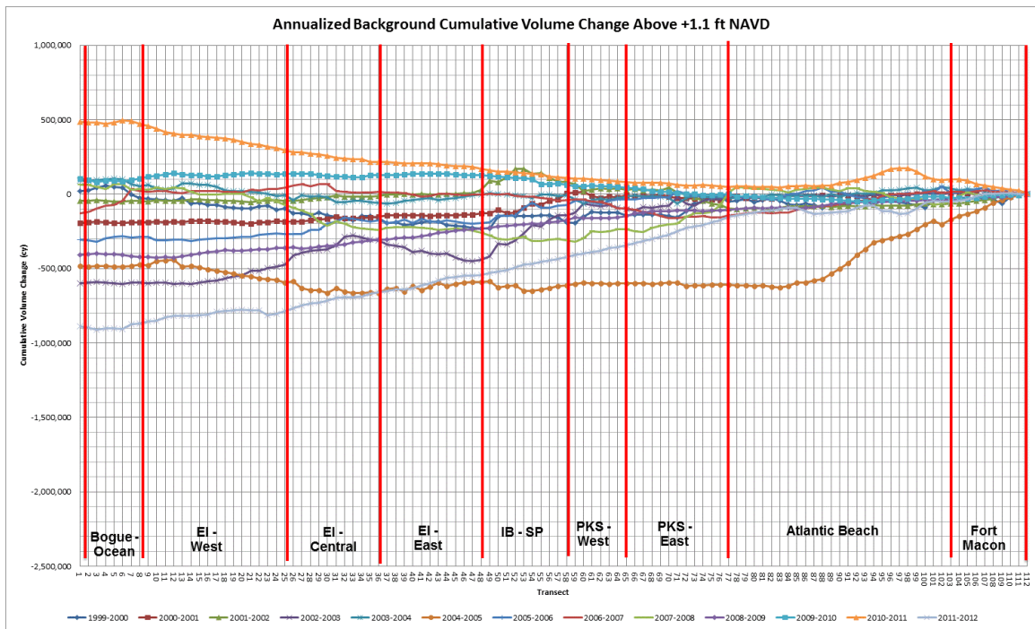
Annualized Background Cumulative Volume Change (Above +1.1 ft NAVD88)
