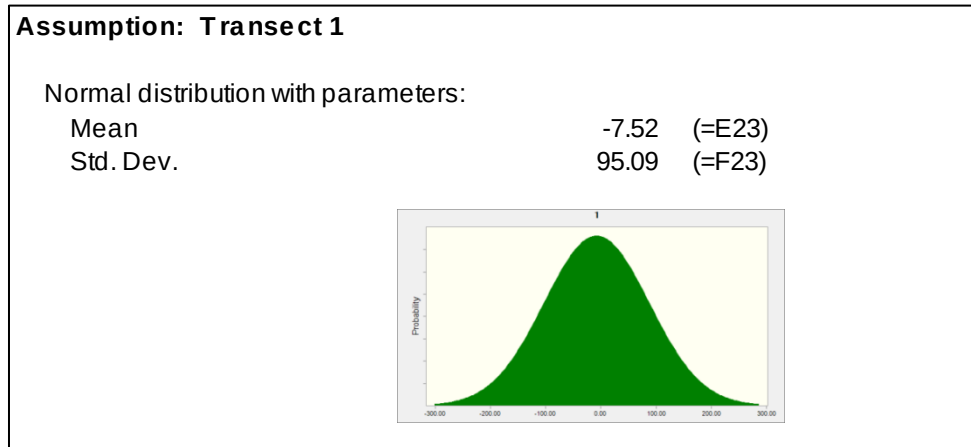
Figure 3: Example Crystal Ball Assumption Input – Transect 1 (-12 ft NAVD88)
