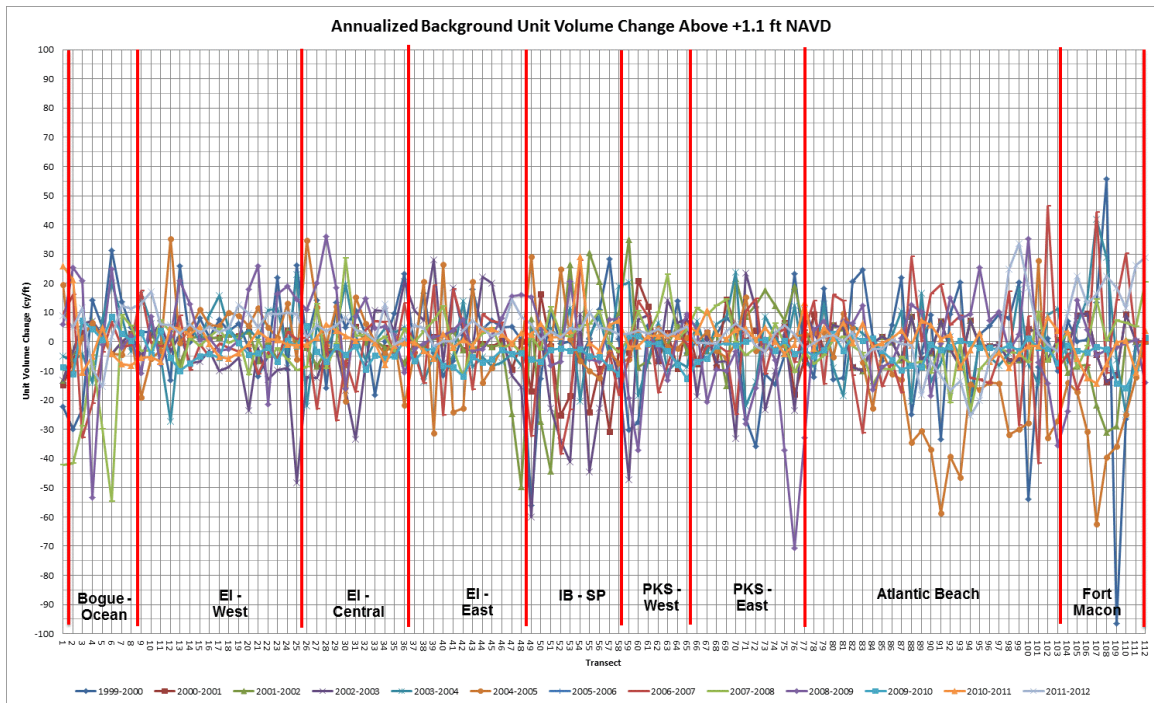
Annualized Background Unit Volume Change (Above +1.1 ft NAVD88)
