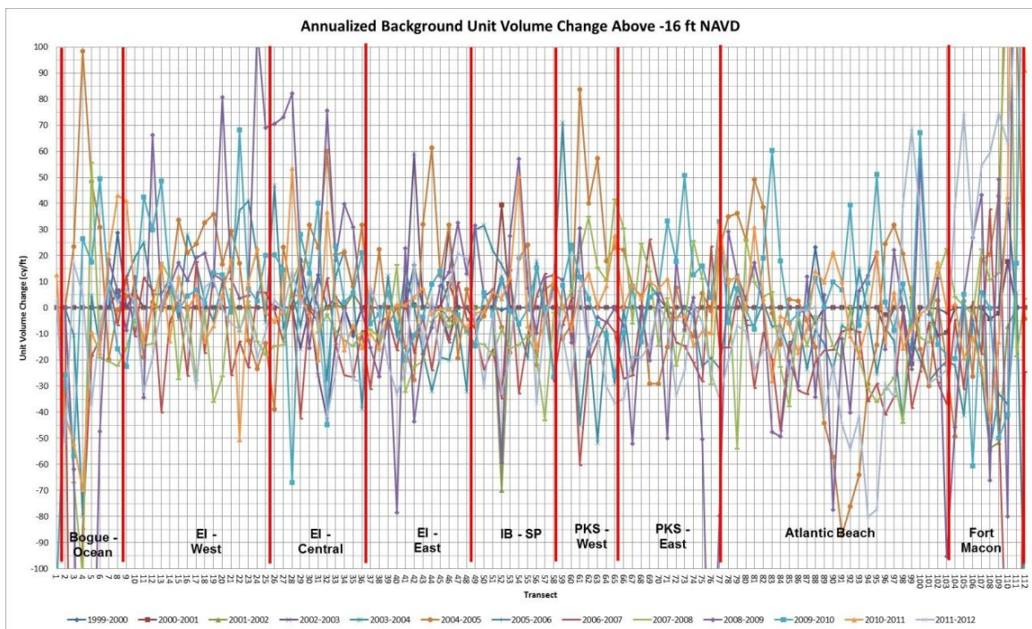
Annualized Background Unit Volume Change (Above -16.0 ft NAVD88)
