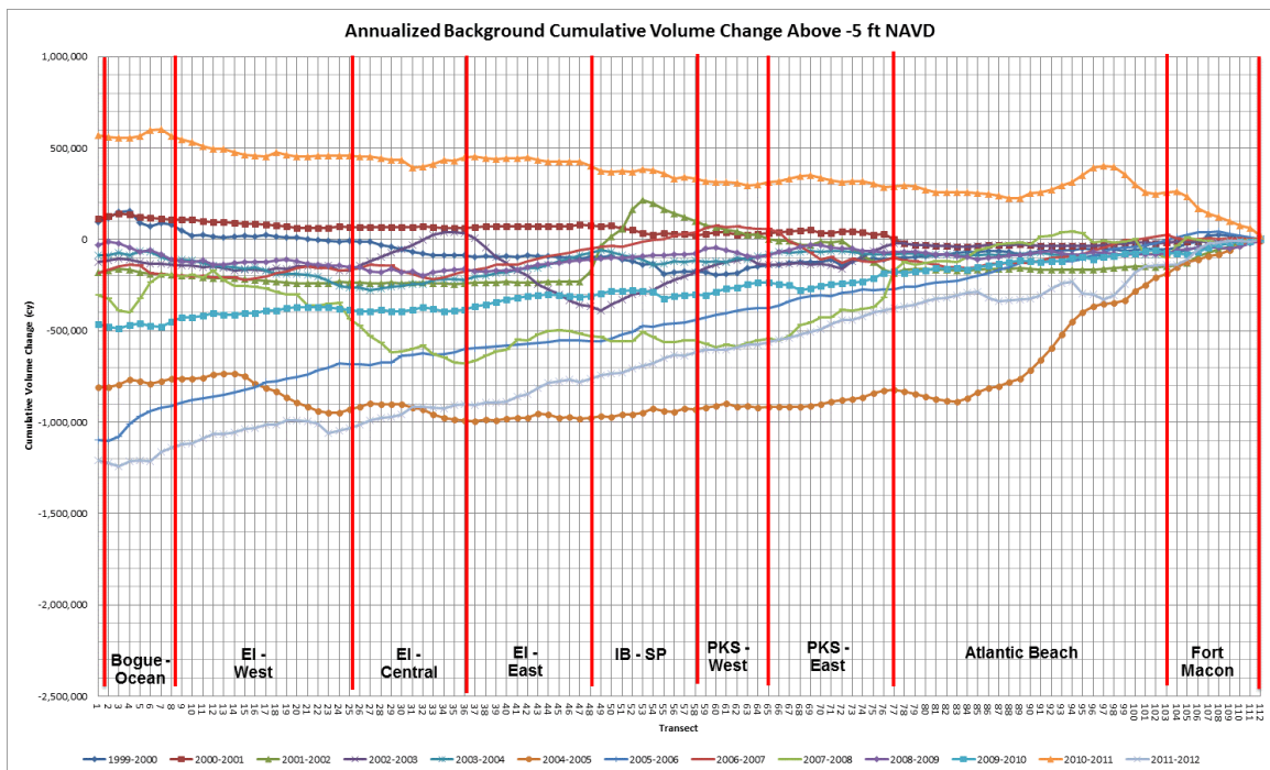
Annualized Background Cumulative Volume Change (Above -5.0 ft NAVD88)
