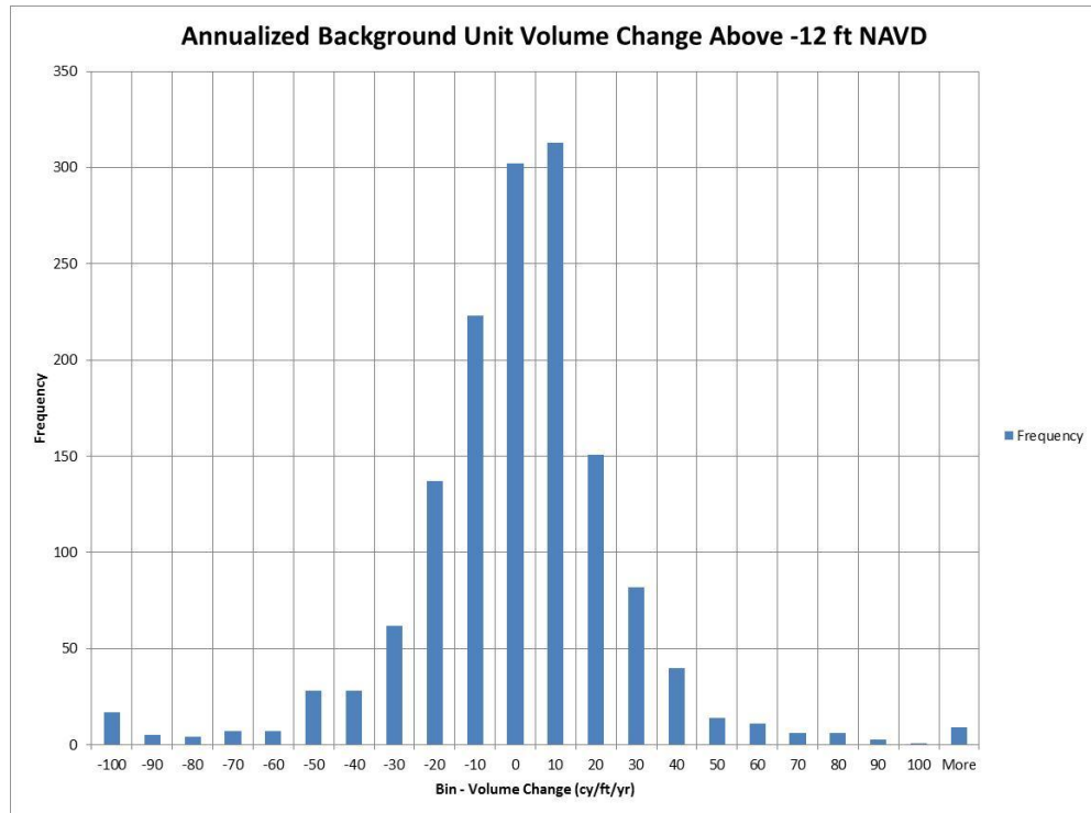
Figure 1: Annualized Background Unit Volume Change (Above -12 ft NAVD88)
