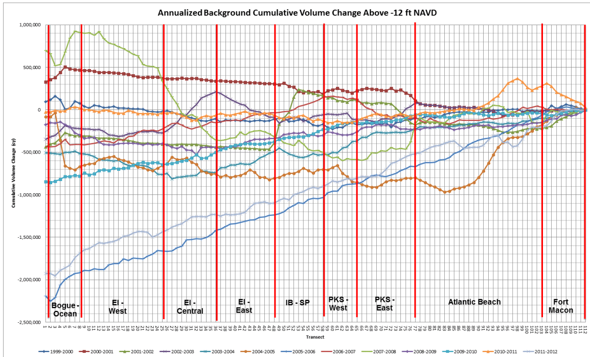
Annualized Background Cumulative Volume Change (Above -12.0 ft NAVD88)
