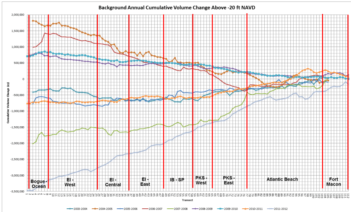
Annualized Background Cumulative Volume Change (Above -20.0 ft NAVD88)
