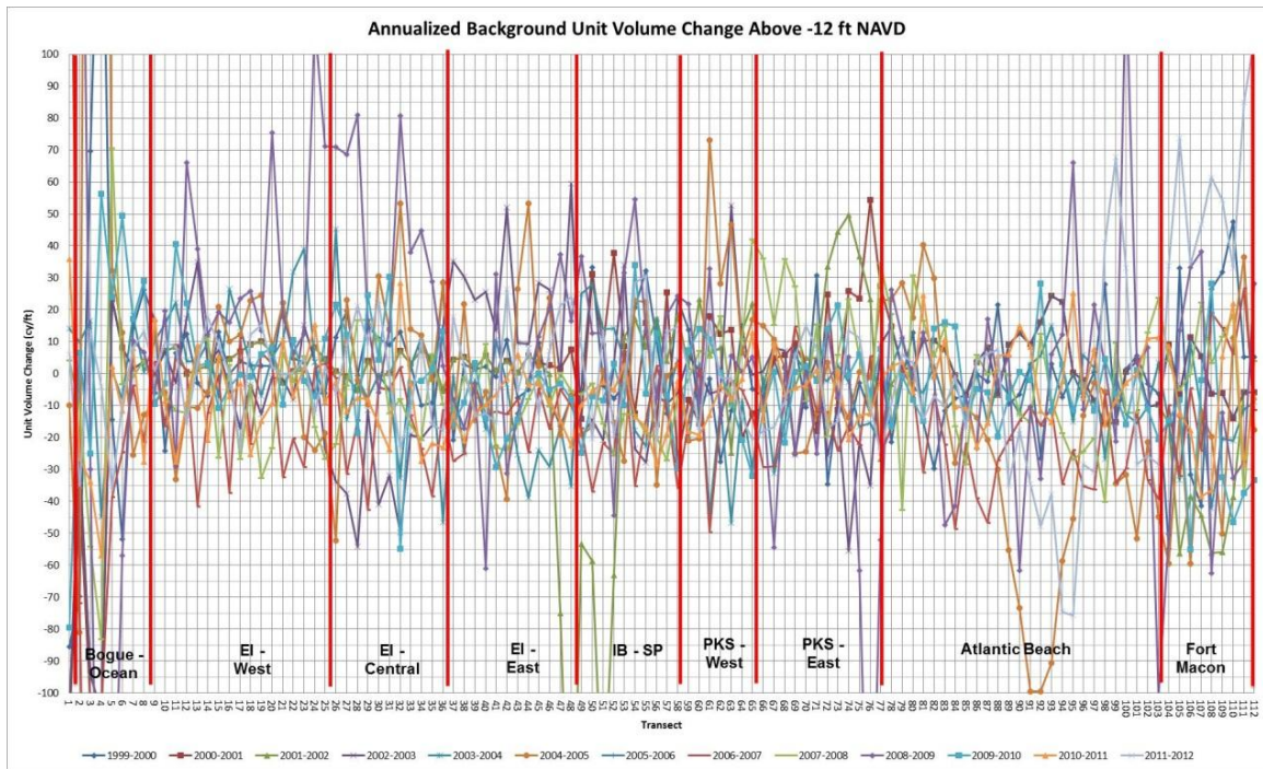
Annualized Background Unit Volume Change (Above -12.0 ft NAVD88)
