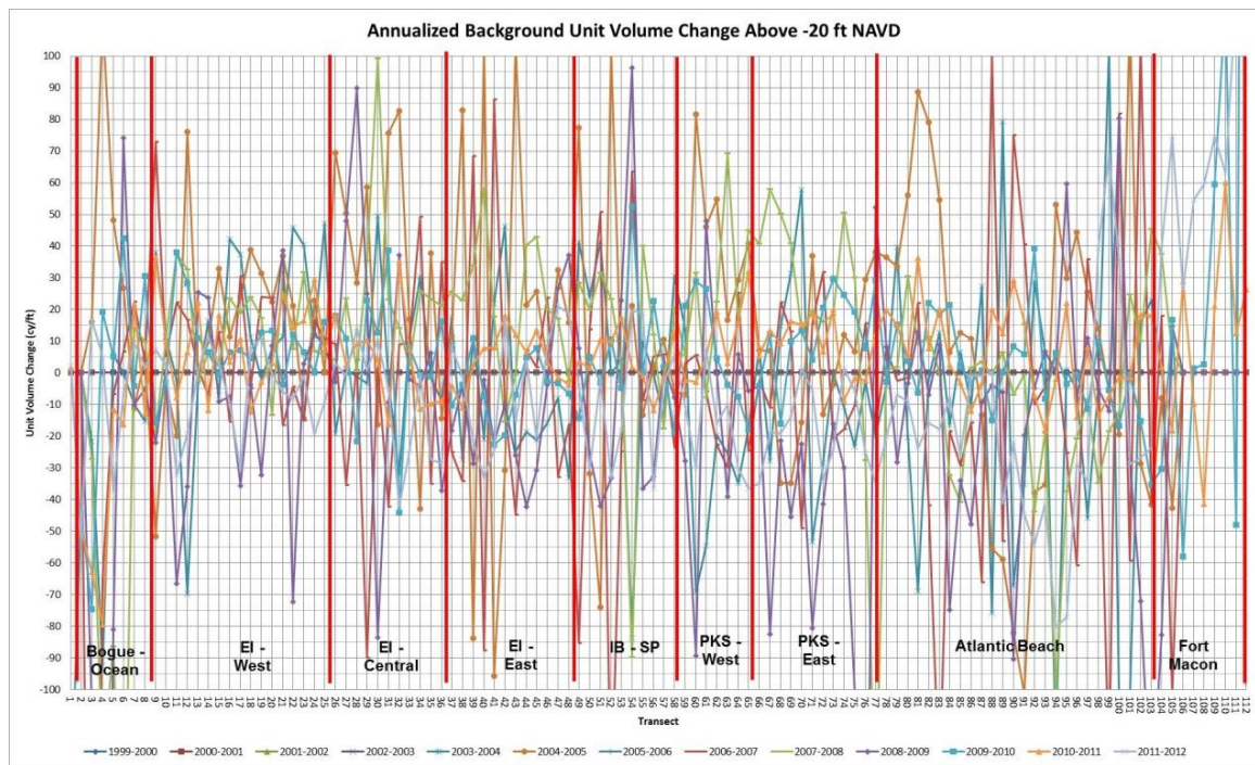
Annualized Background Unit Volume Change (Above -20.0 ft NAVD88)
