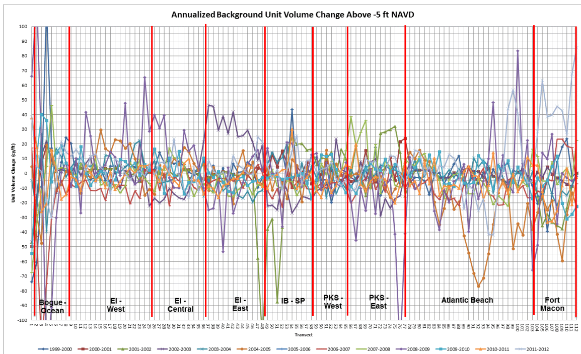
Annualized Background Unit Volume Change (Above -5.0 ft NAVD88)
