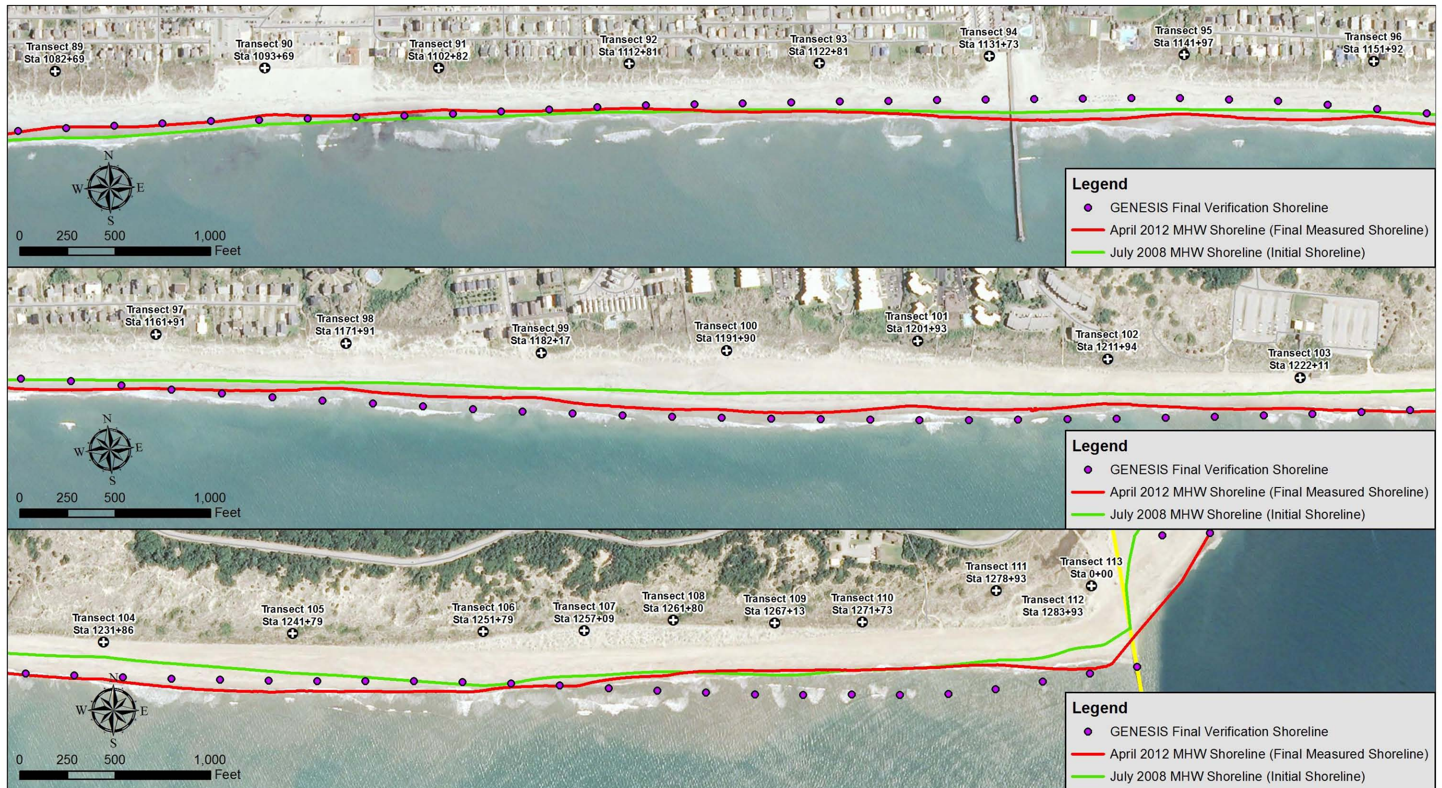
Figure 2-6. GENESIS-T Verification Results (Transects 89-112)
