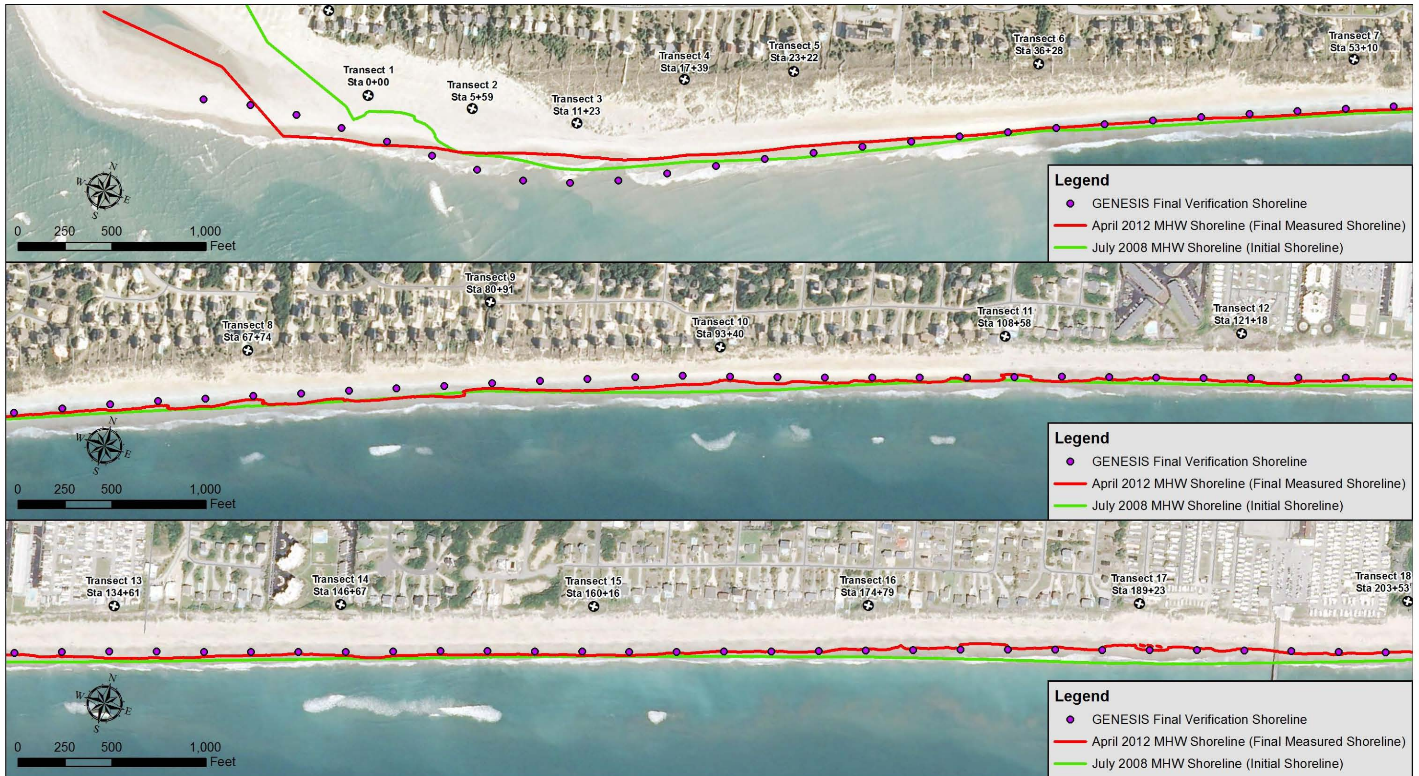
Figure 2-1. GENESIS-T Verification Results (Transects 1-18)
