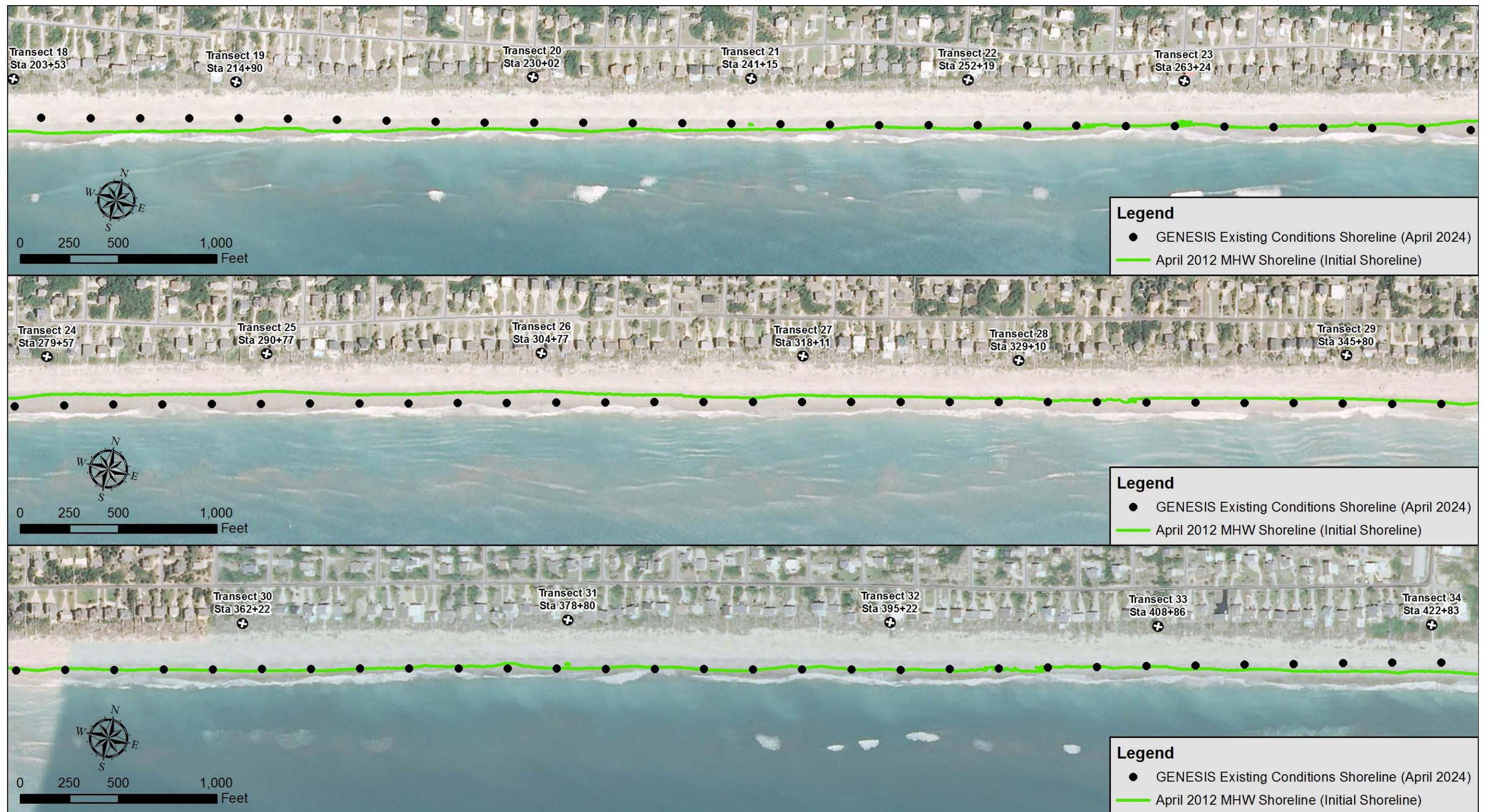
Figure 3-2. GENESIS-T Existing Conditions Results (Transects 18-34)
