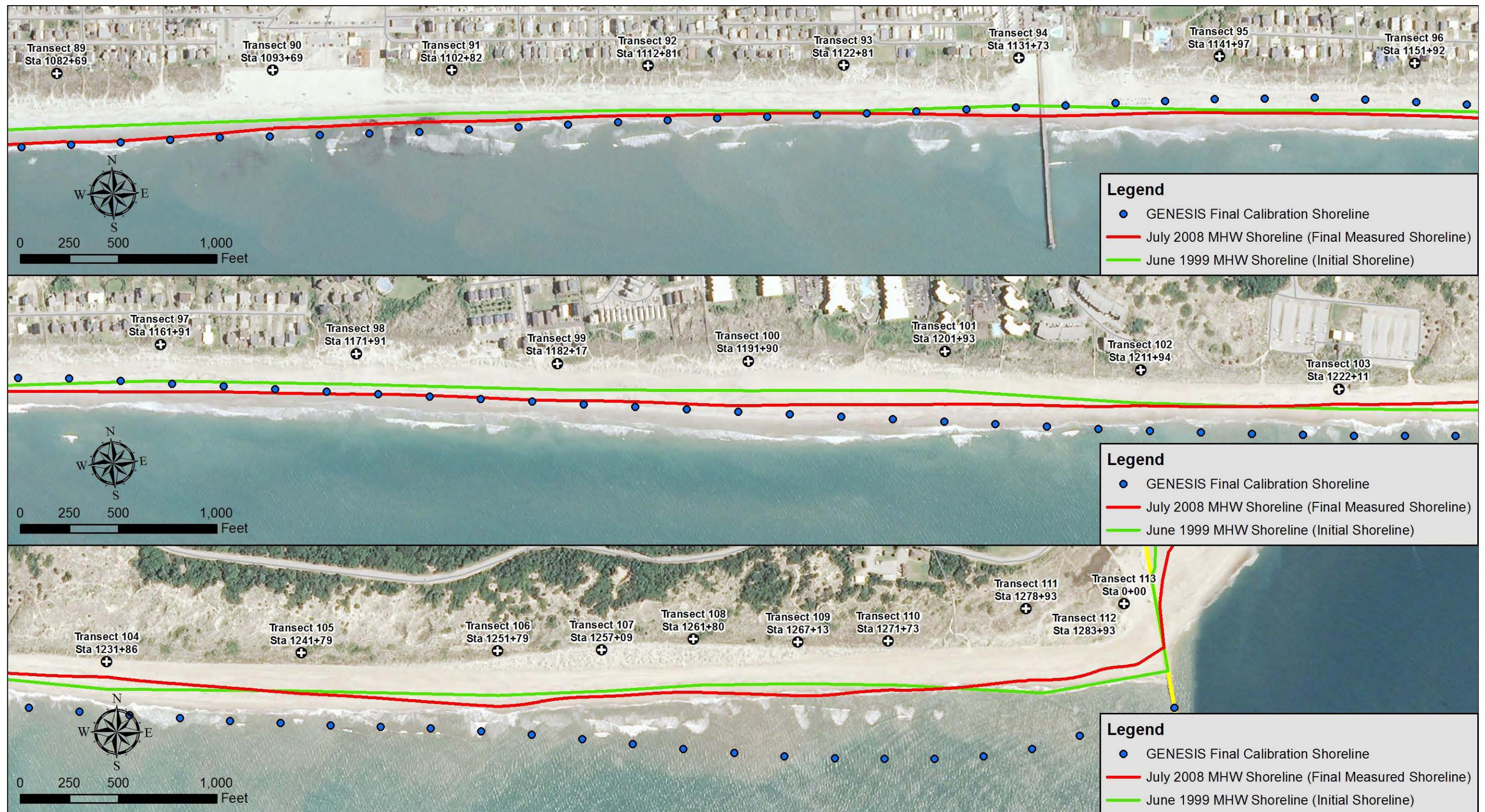
Figure 1-6. GENESIS-T Calibration Results (Transects 89-112)
