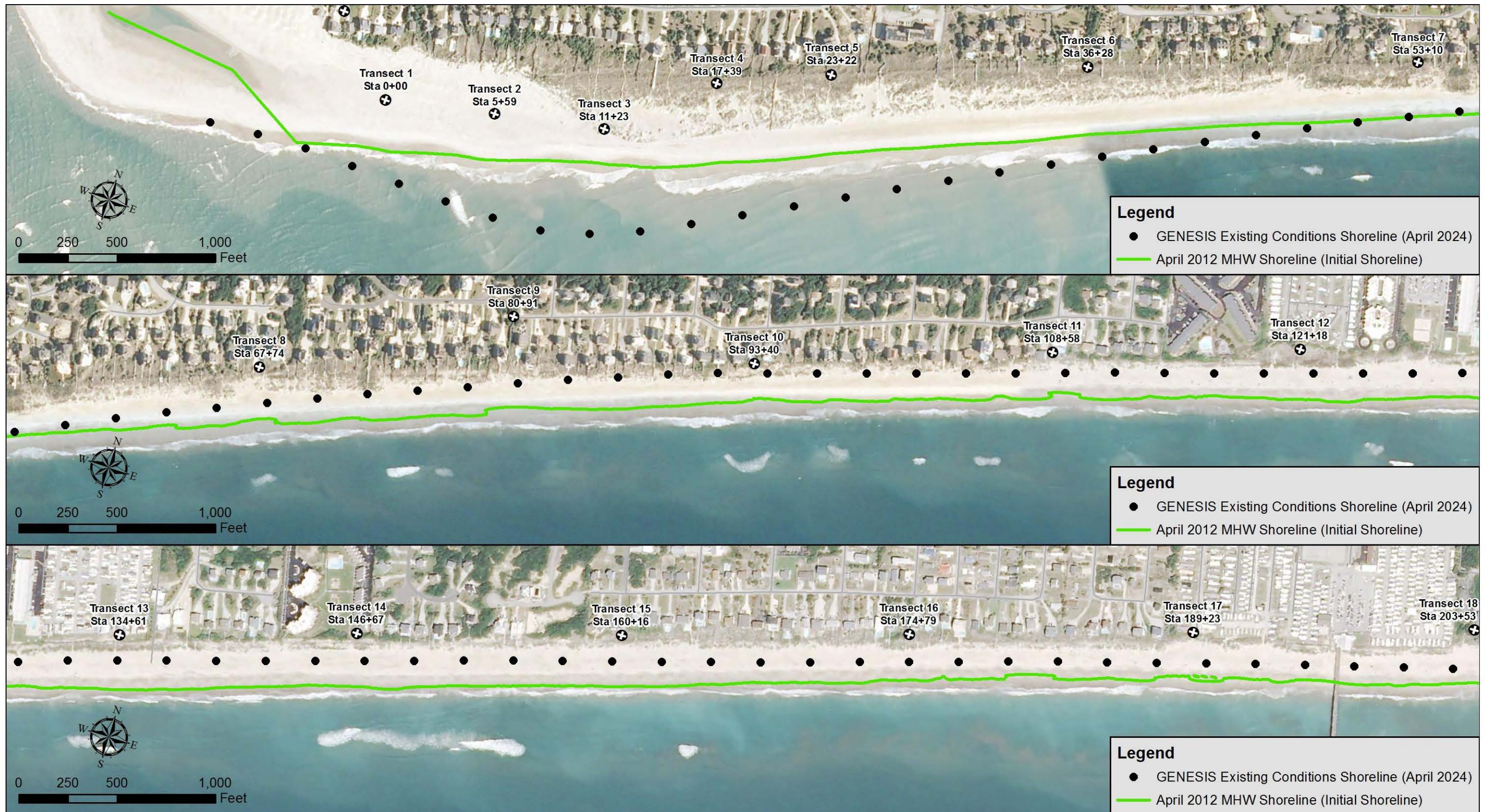
Figure 3-1. GENESIS-T Existing Conditions Results (Transects 1-18)
