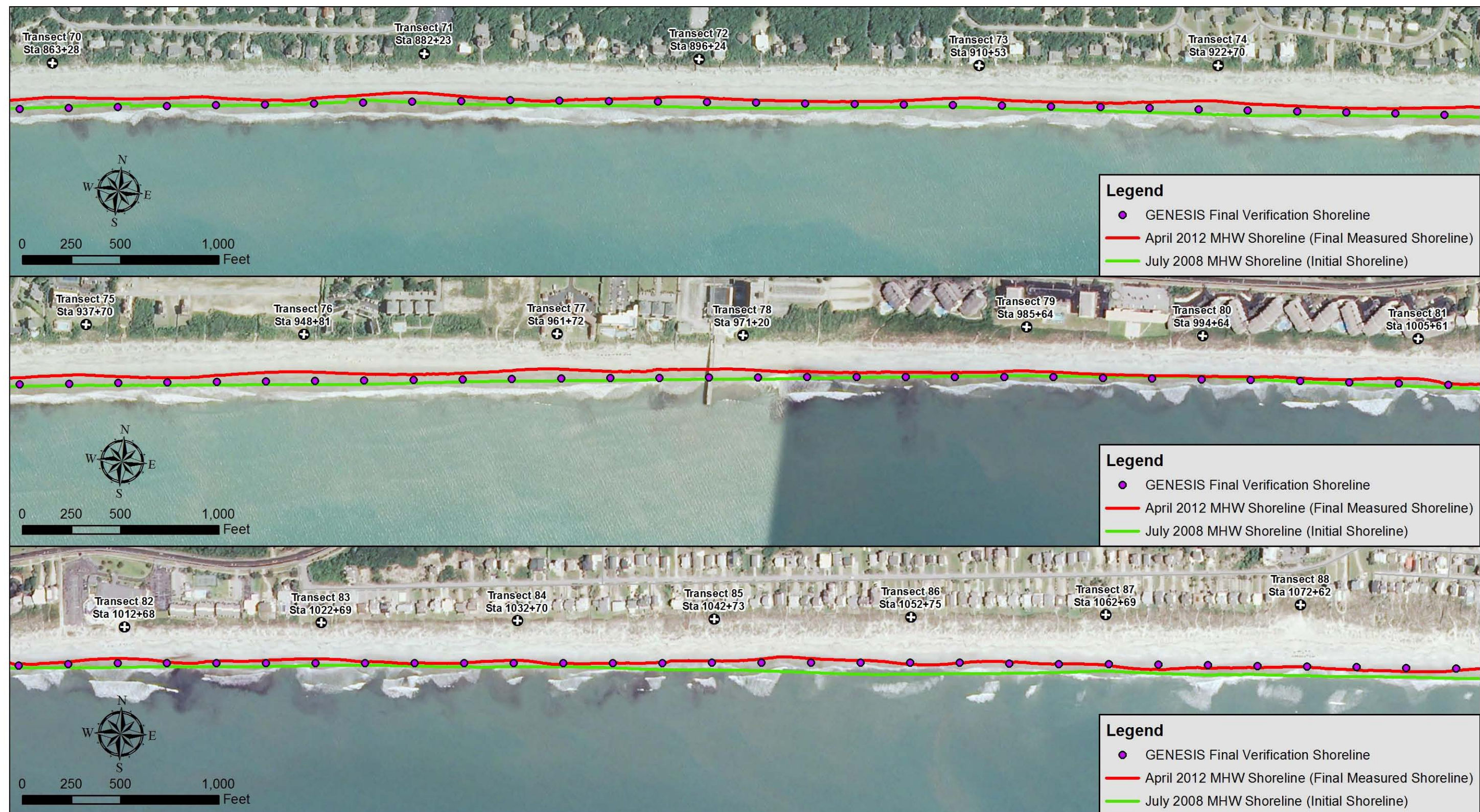
Figure 2-5. GENESIS-T Verification Results (Transects 70-88)
