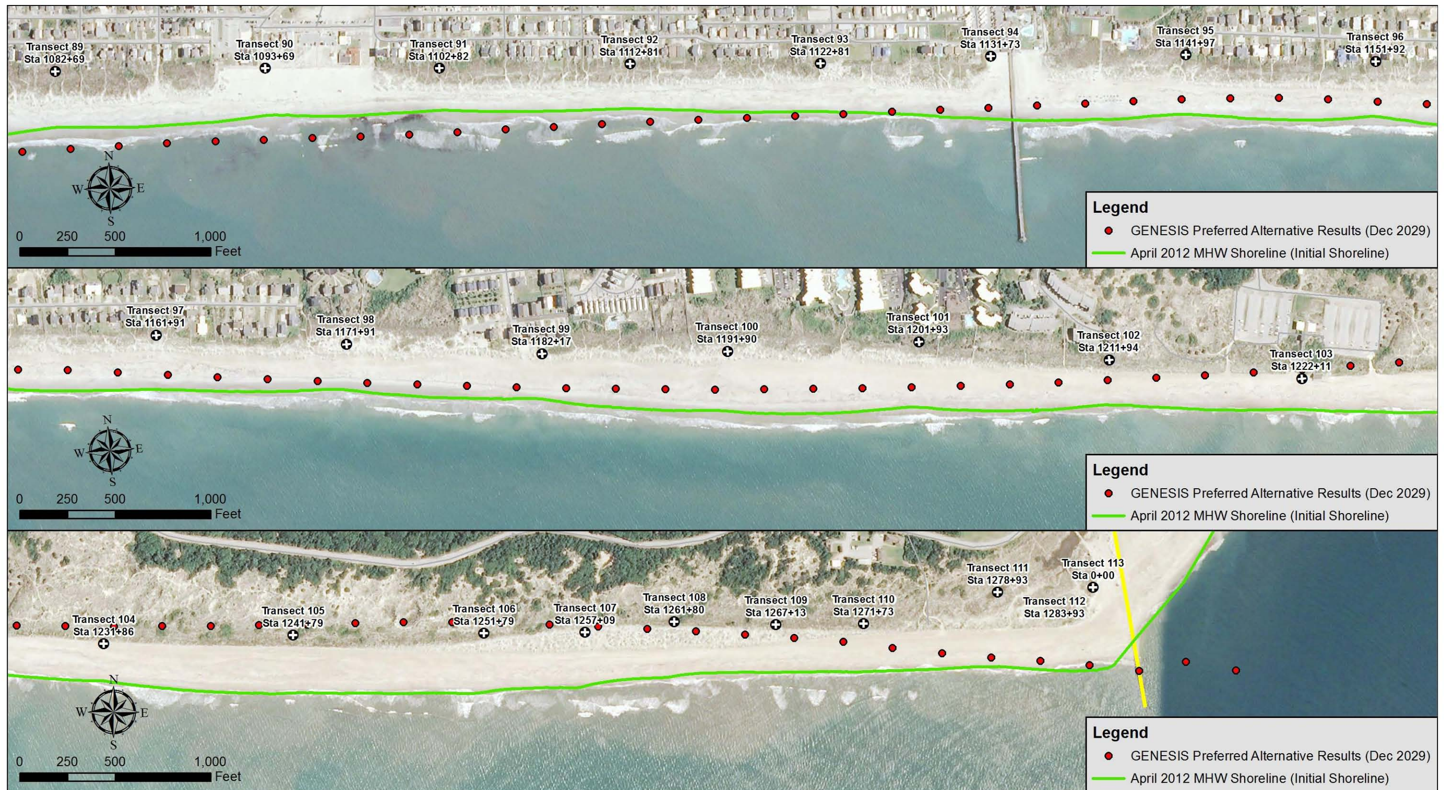
Figure 4-6. GENESIS-T Preferred Alternative Results (Transects 89-112)
