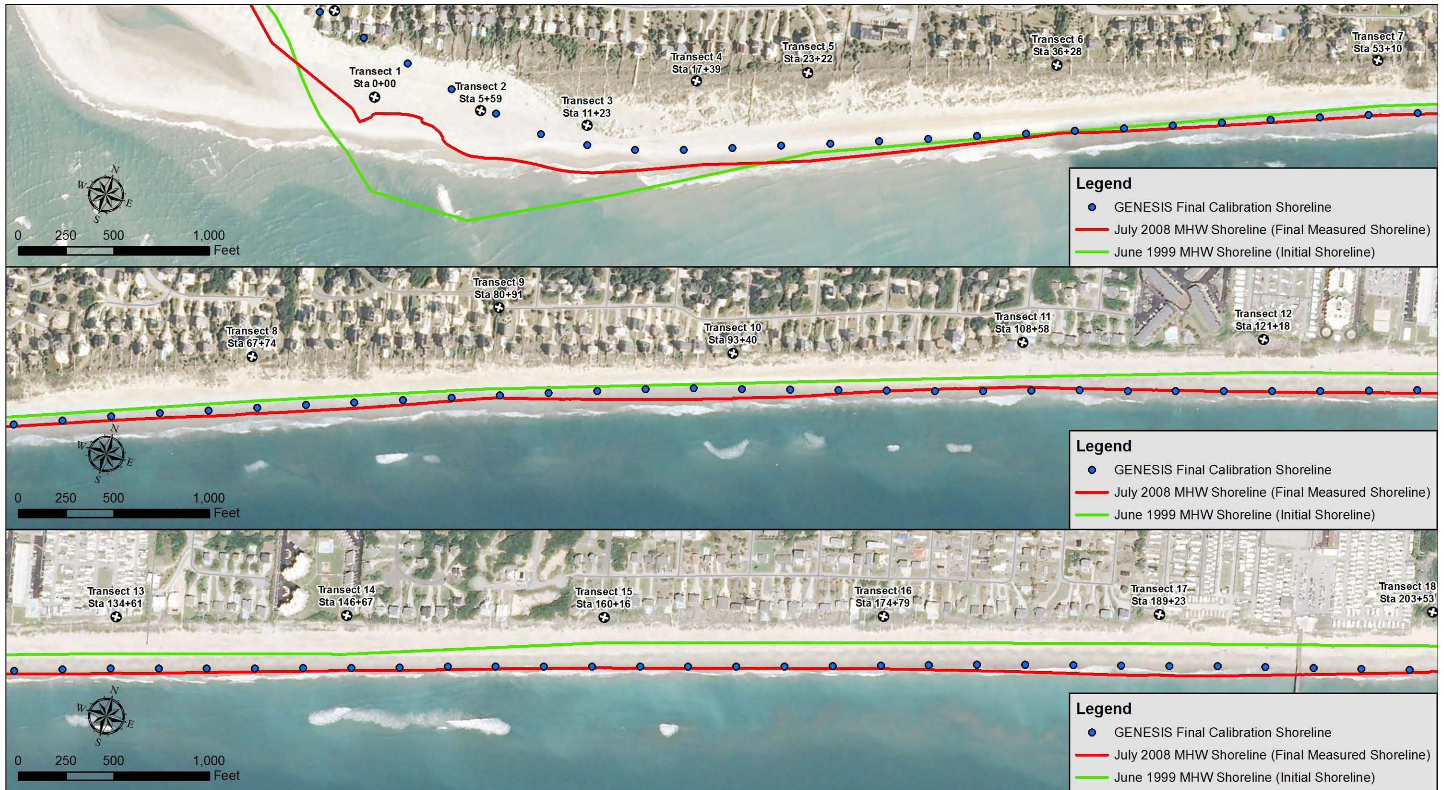
Figure 1-1. GENESIS-T Calibration Results (Transects 1-18)
