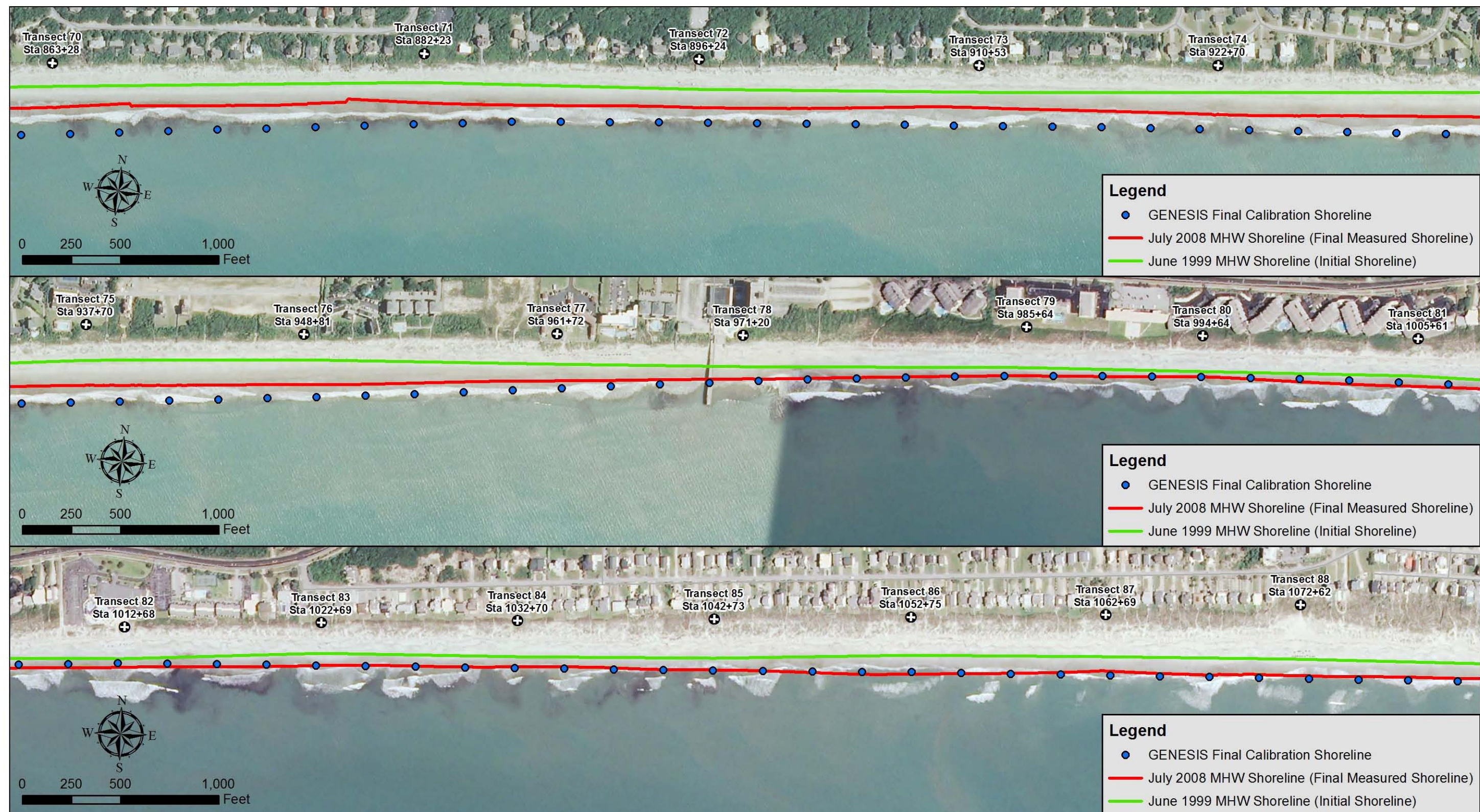
Figure 1-5. GENESIS-T Calibration Results (Transects 70-88)
