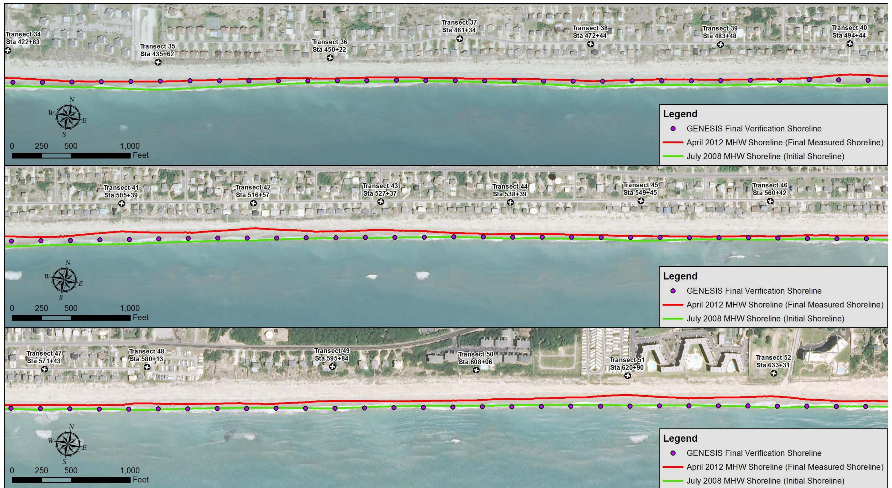
Figure 2-3. GENESIS-T Verification Results (Transects 34-52)
