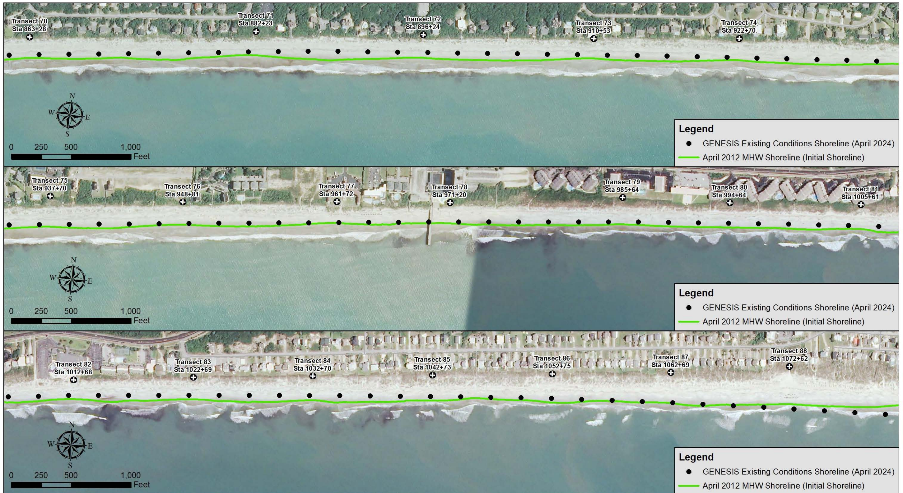
Figure 3-5. GENESIS-T Existing Conditions Results (Transects 70-88)
