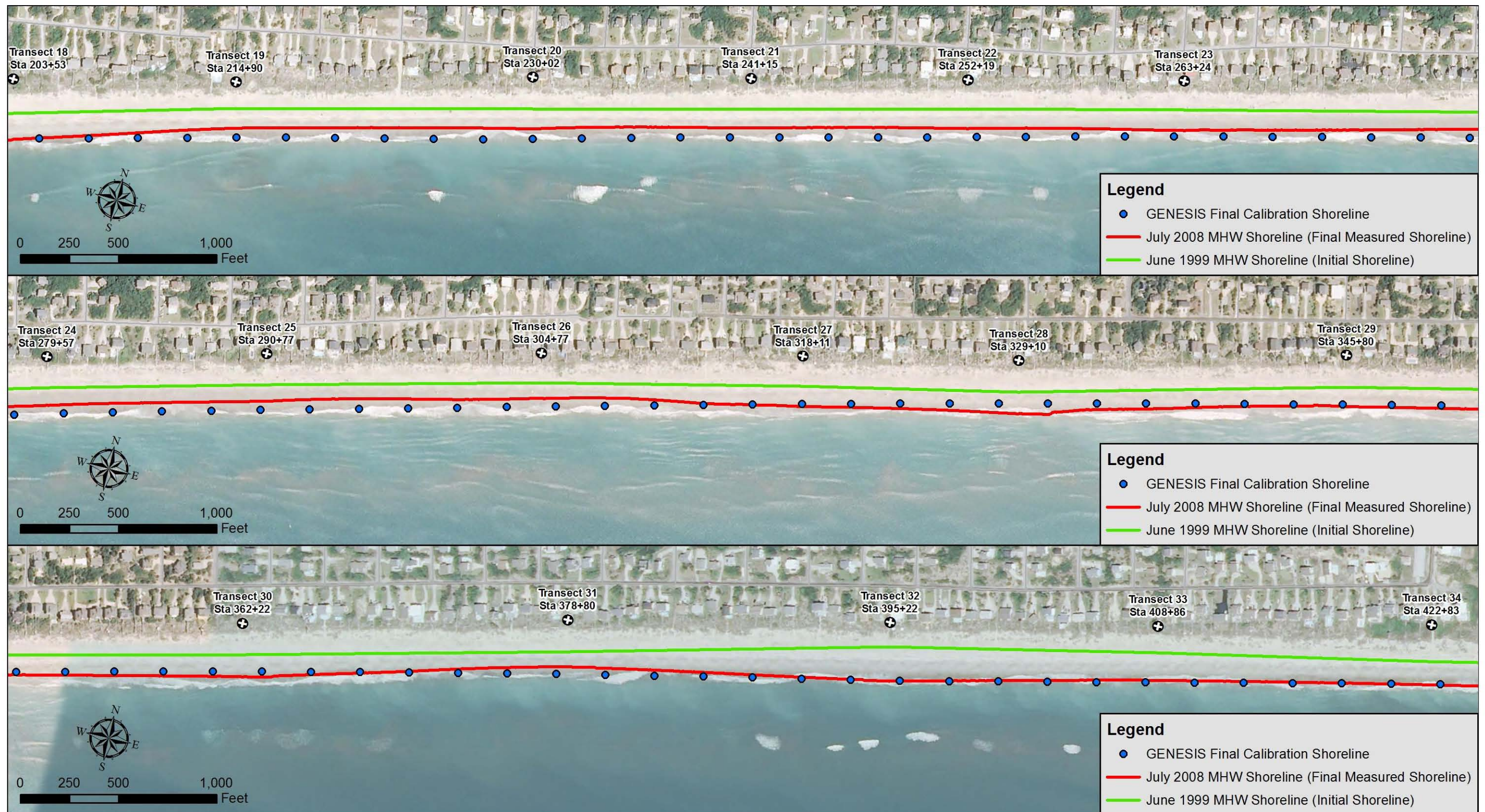
Figure 1-2. GENESIS-T Calibration Results (Transects 18-34)
