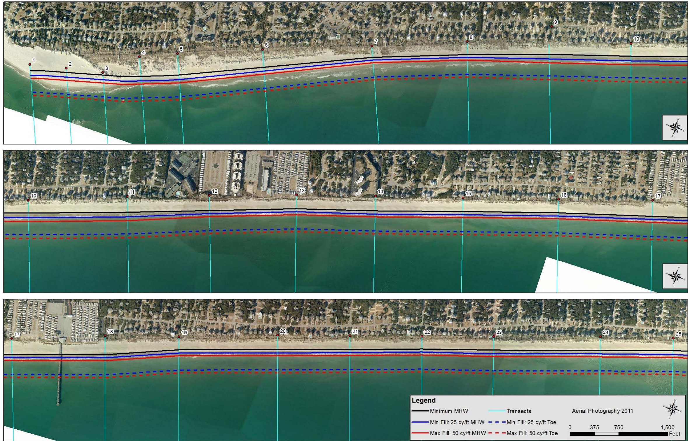
Figure 1. Preferred Alternative Plan View (Transects 1-25)
