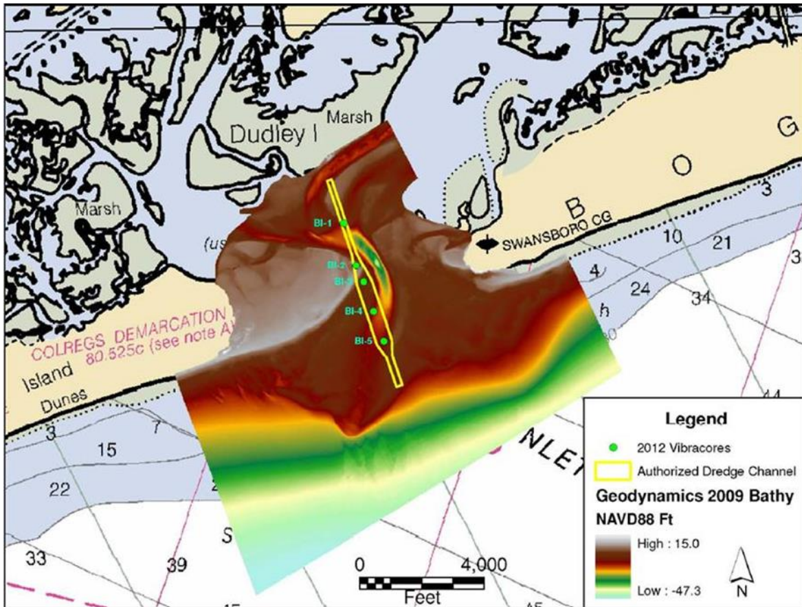
Figure 3.15. Bogue Inlet Proposed Ebb Channel Realignment Footprint with Vibracore Locations
