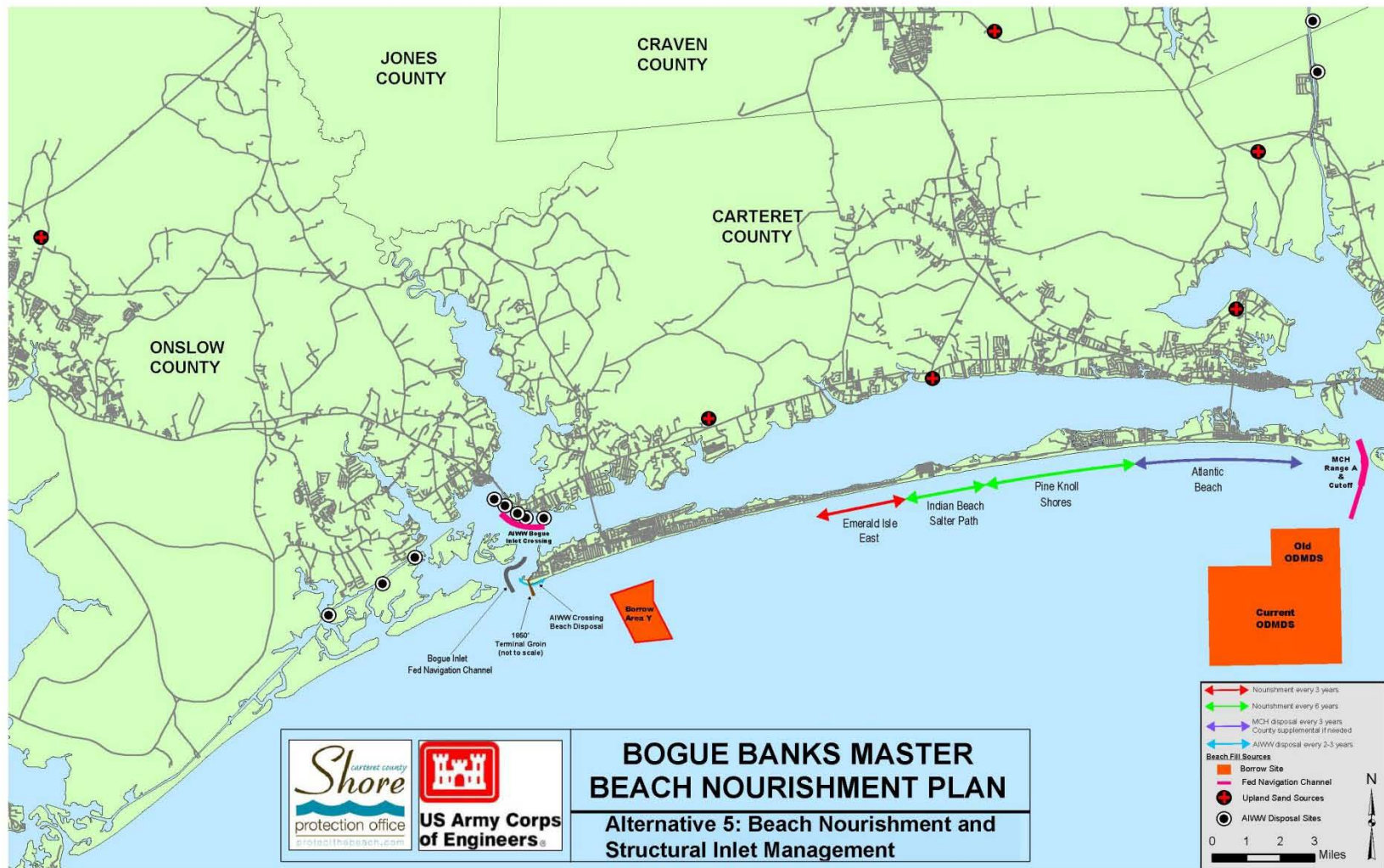
Figure 3.16. Alternative 5 - Nourishment with Structural Inlet Management
