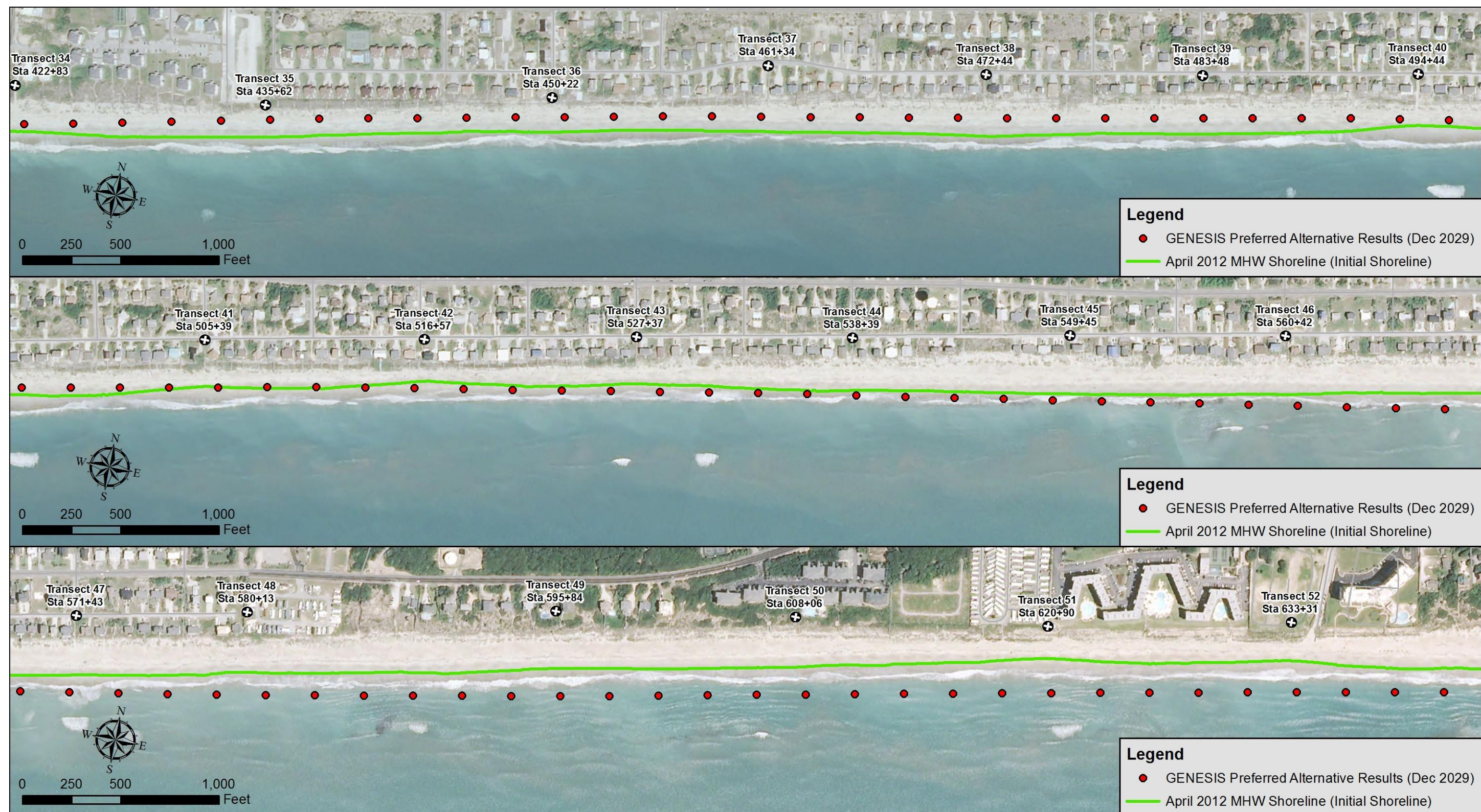
Figure 4-3. GENESIS-T Preferred Alternative Results (Transects 34-52)
