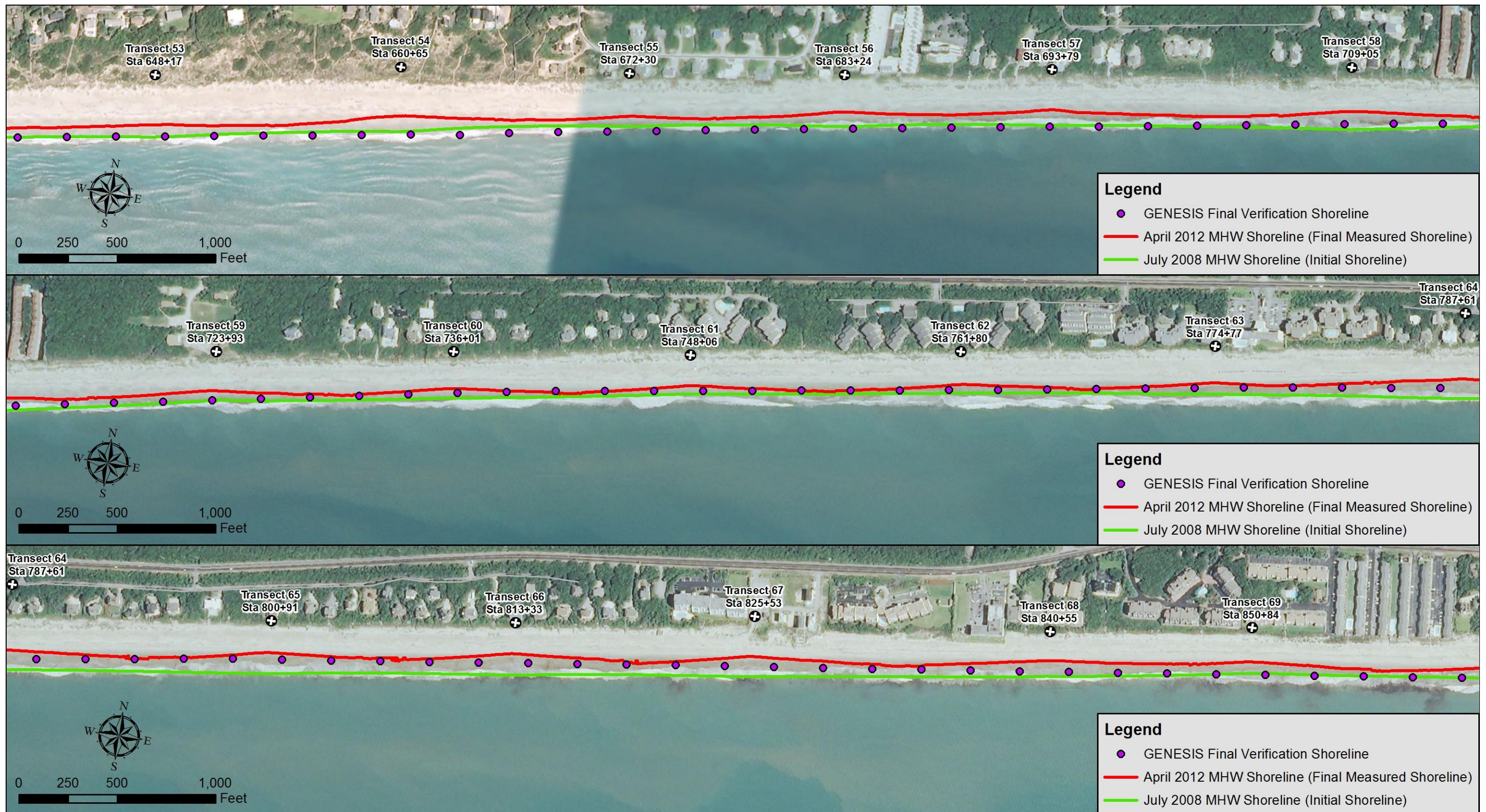
Figure 2-4. GENESIS-T Verification Results (Transects 53-69)
